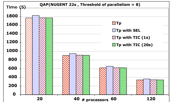
Fig. 8. Execution Times of Protocols.
