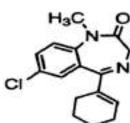
Tetrazeepam
