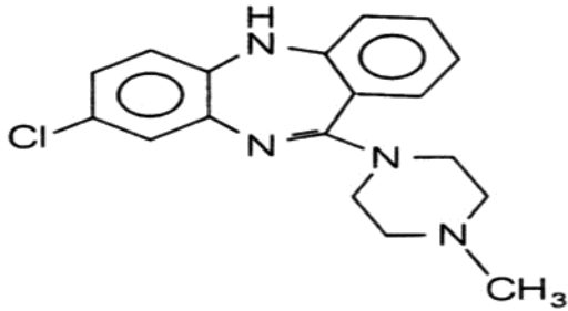
Clozapine
