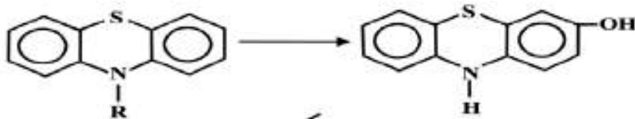
Hydroxyphenothiazine
