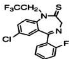
Quazepam
